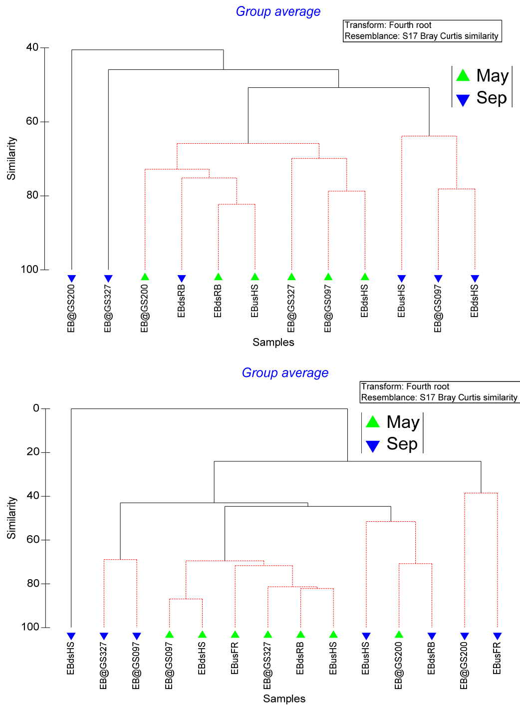
Figure 3-14 Cluster analysis of Fyke samples (upper panel) and electrofishing samples (lower panel) September samples with corresponding May/June samples.
