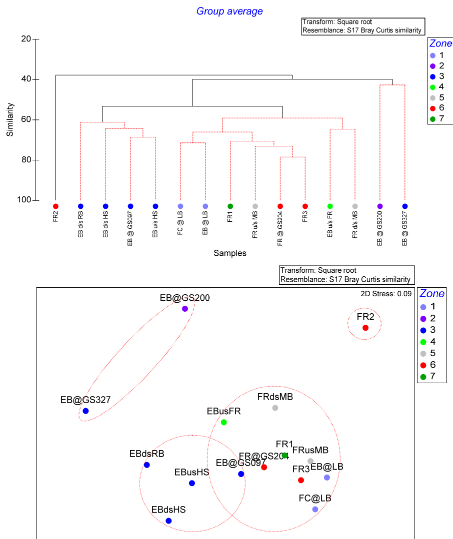
Figure 3-6 Cluster analysis (upper panel) and nMDS plot (lower panel) of macroinvertebrate communities. Red circles indicate significant cluster groups.
