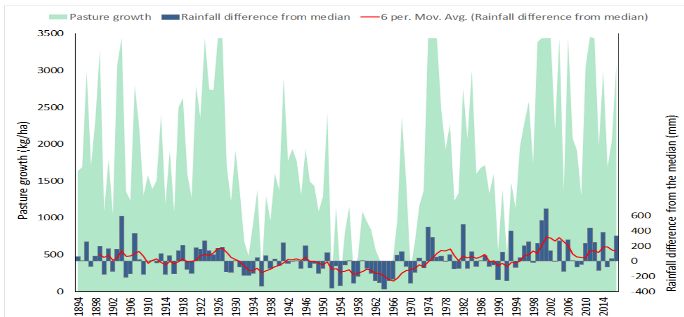
Figure 10: Modelled pasture growth and rainfall (difference each year from the long term median) over time on an alluvial land type in the southern VRD.
