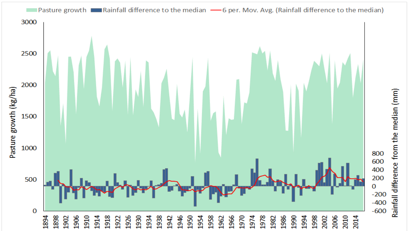
Figure 11: Modelled pasture growth and rainfall (difference each year from the long term median) over time on the Banjo land system at Larrimah.
